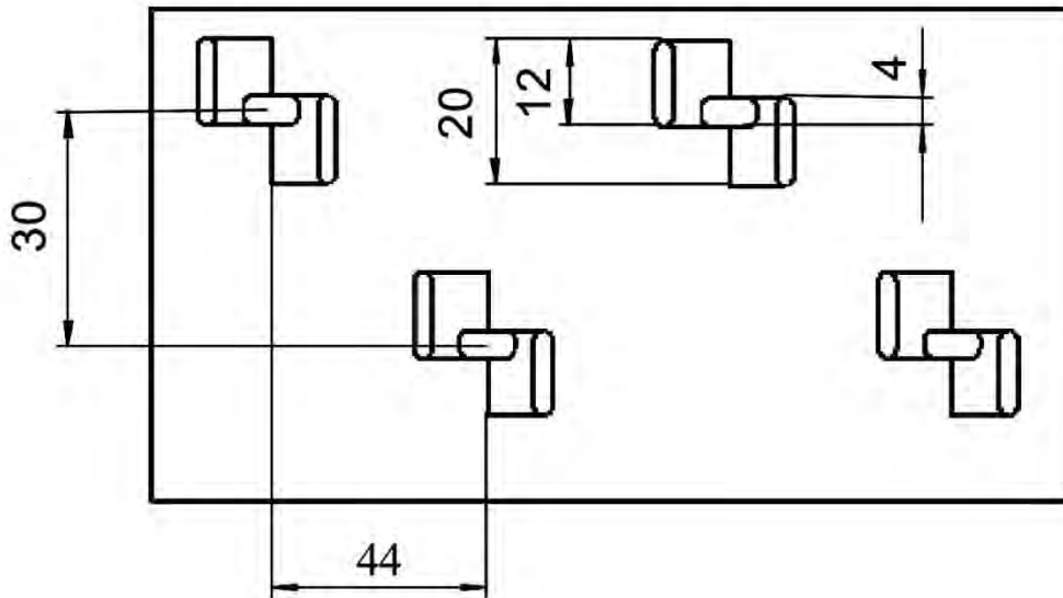
Arrangement of anchor studs (Guide values in mm)
