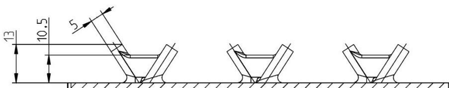
(Guide values in mm)
