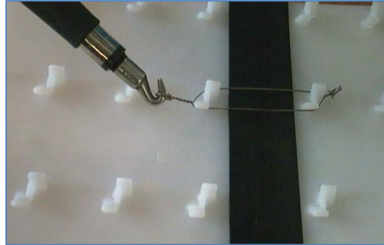
(Example: Connection of CPL by means of wire loops at every 6 th row of studs)
